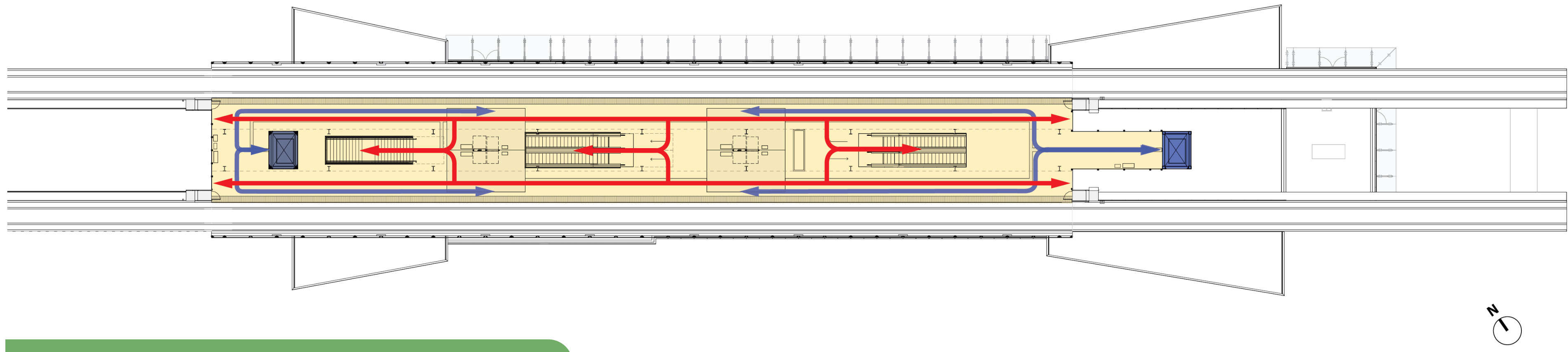
Platform floor plan
